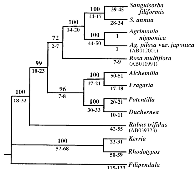
Fig. 2 Most parsimonious tree based on matK sequences for Rosoideae s.s. Bootstrap percentages, based on 1000 replicate analyses, are shown above nodes. Possible length from minimum to maximum is shown below each node
